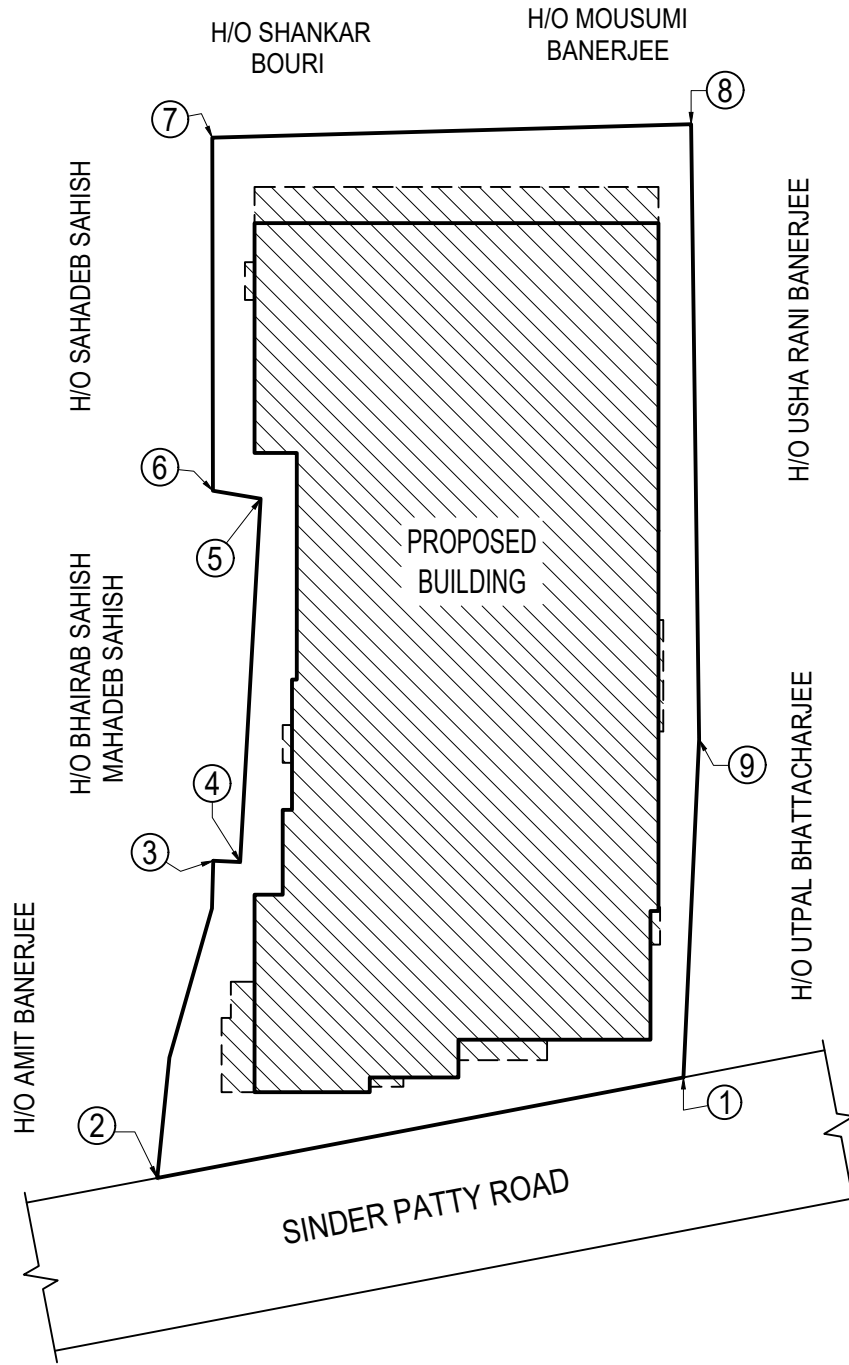
SITE PLAN
